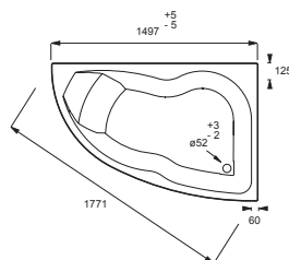
Micromega Duo - Corner bath
