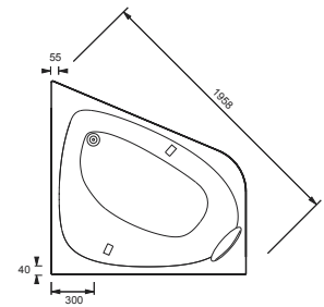
Reach - Corner bath
