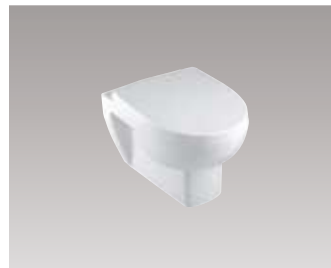
Reach - Wall-hung WC pan with CLEAN technology 54 x 36.5 cm low flush 2.6/4 L or 3/6 L possible 4970K Order toilet seat separately: 8322K - Slim removable WC seat with slow-close 8409K - removable WC seat with slow-close 8407K - standard WC seat
