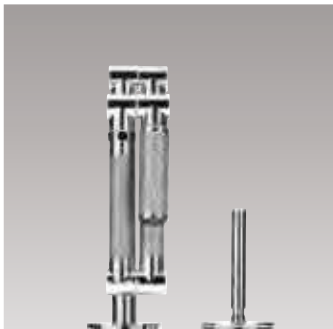
Karbon Articulating single control tap with "joystick" control positioned left or right 2 spray options: Laminar and aerated Fold-up height 228 mm, maximum reach 337 mm
