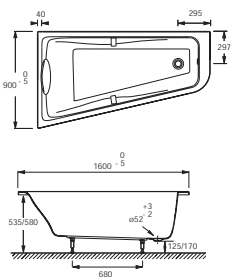
Reach - Offset bath
